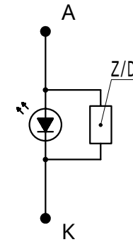
Internal Circuit
